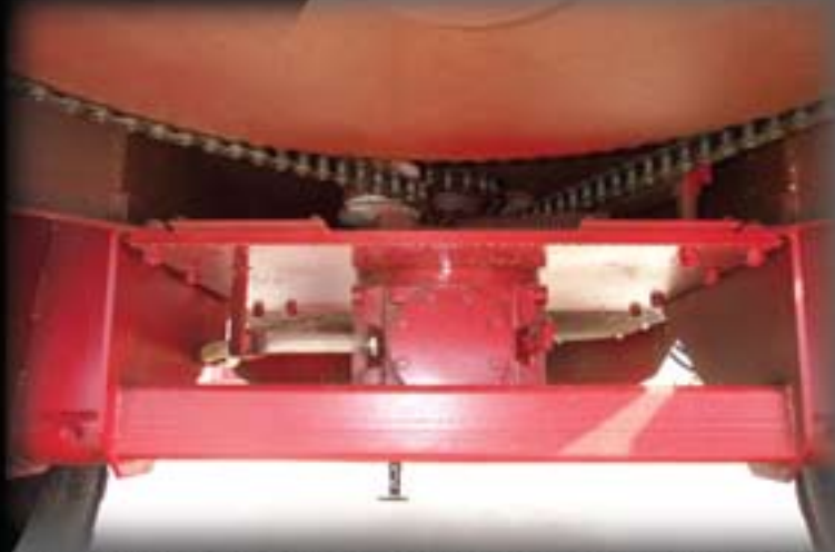
Low Maintenance Chain and Sprocket Drive with One Right Angle Gearbox
